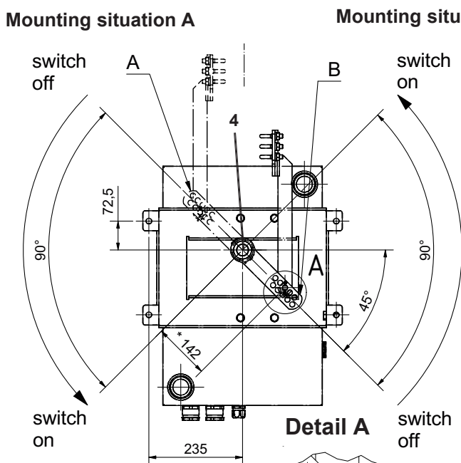
Fig. 6: Mounting the operating crank acc. to mounting situation
