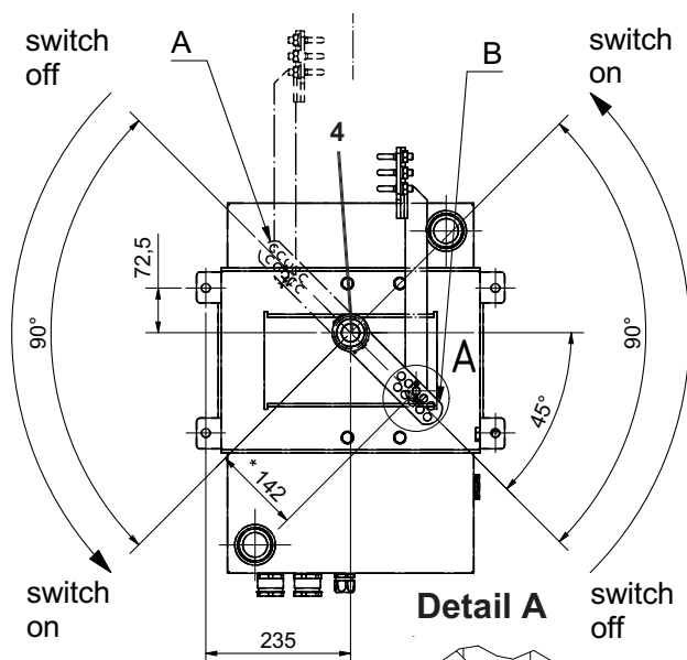
Fig. 6: Mounting the operating crank acc. to mounting situation
